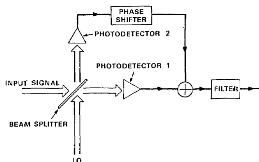
Fig. 1. Schematic for homodyne and heterodyne detection: the beam splitter is assumed lossless with power transmission \epsilon and reflection 1 - \epsilon .
